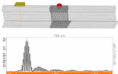
Inspection Simulation on a flawed rail and associated A-scan
