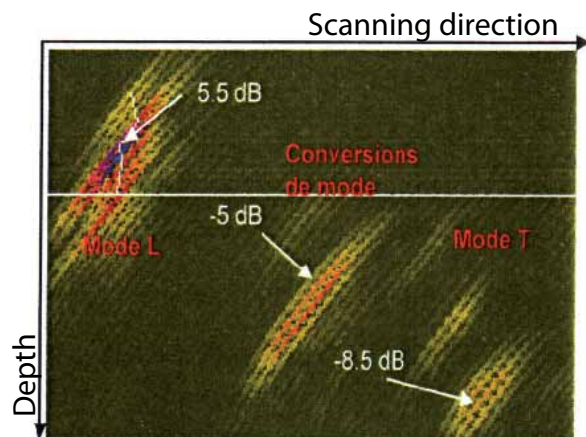
Experimental B-scan showing multiple echoes. The echo labels are an interpretation assuming the crack shape shown below.
