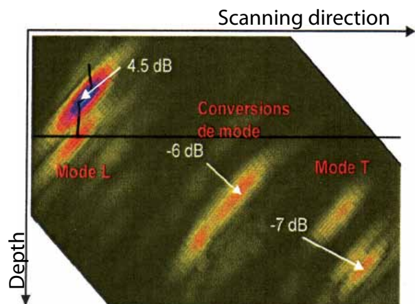
CIVA simulated B-scan corresponding to the crack shape shown in the drawing. The simulated results show excellent correlation to the experimental results, verifying the postulated crack shape
